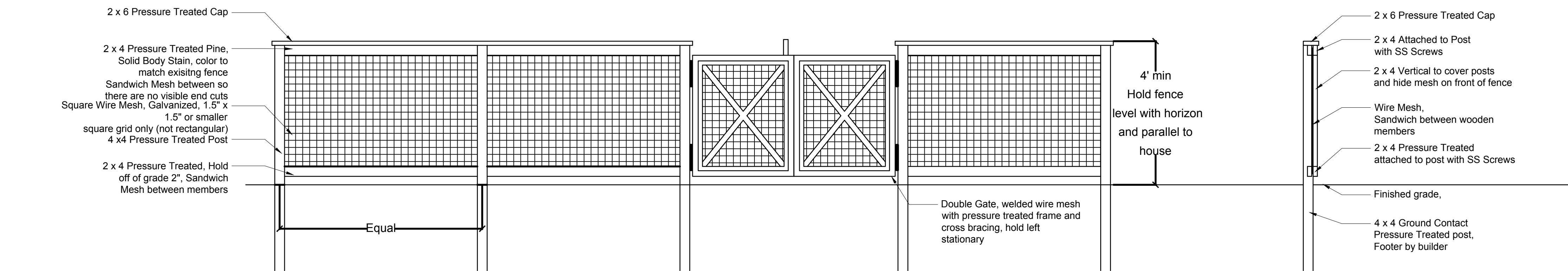
Living Fence and Gate Details: Scale 1/2" = 1'-0"
