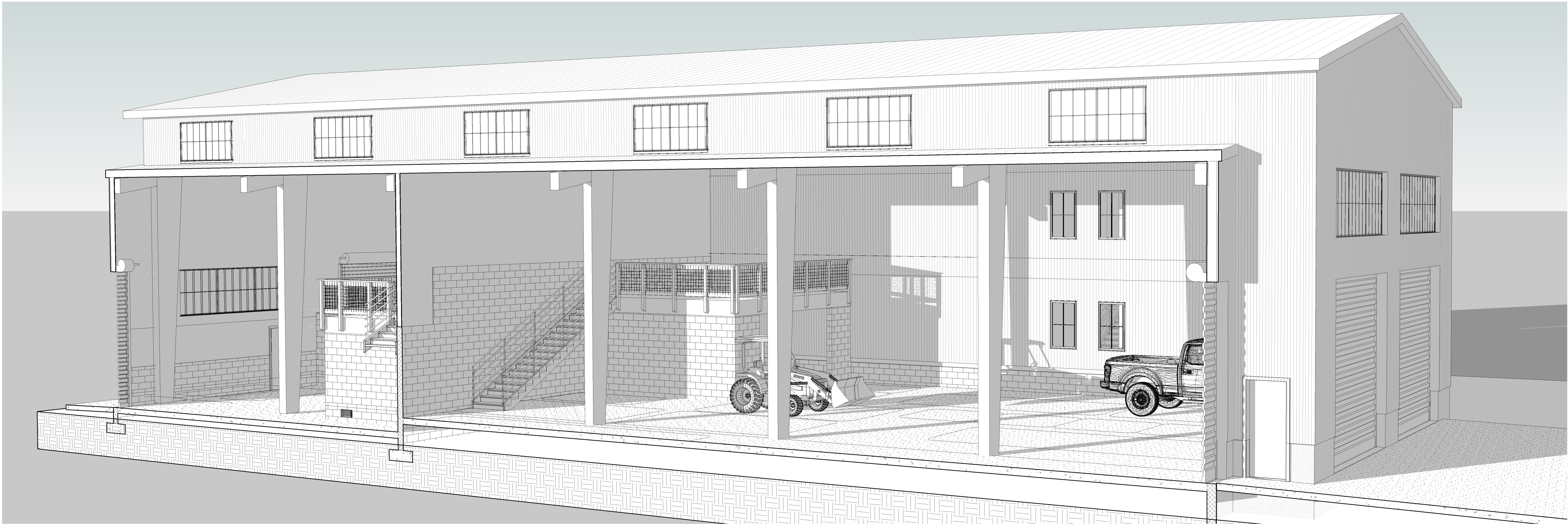
1 TRAN VIEW SECT FROM WEST 01
