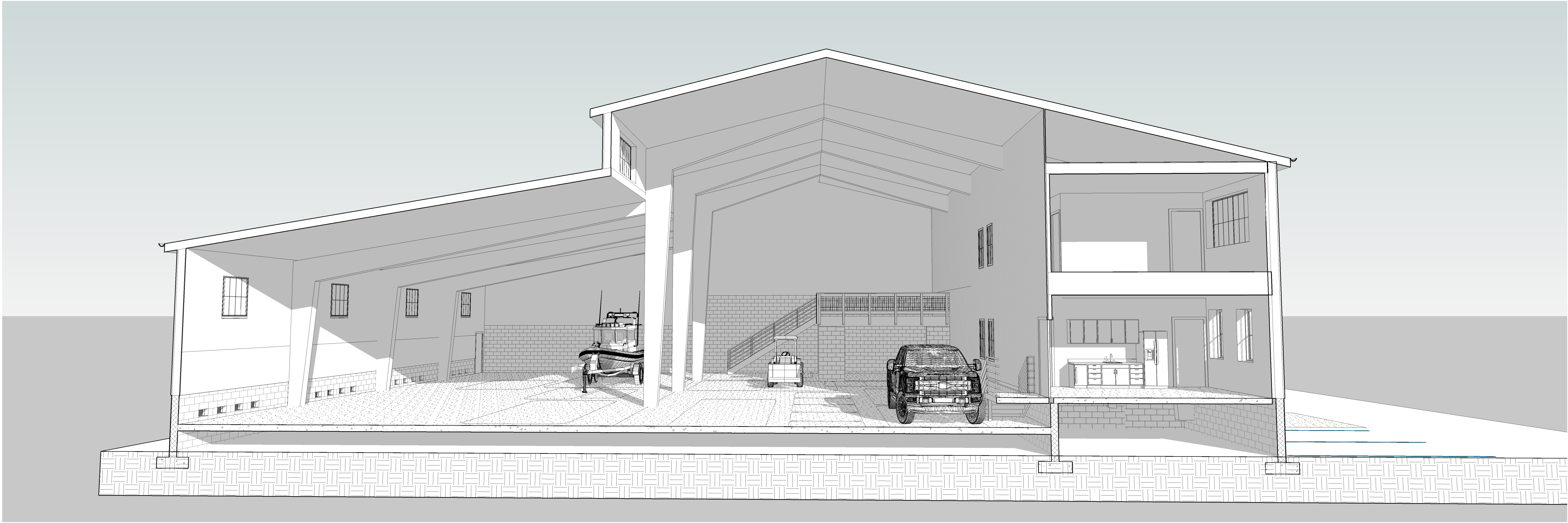
1 LONG VIEW SECT FROM SOUTH 02
