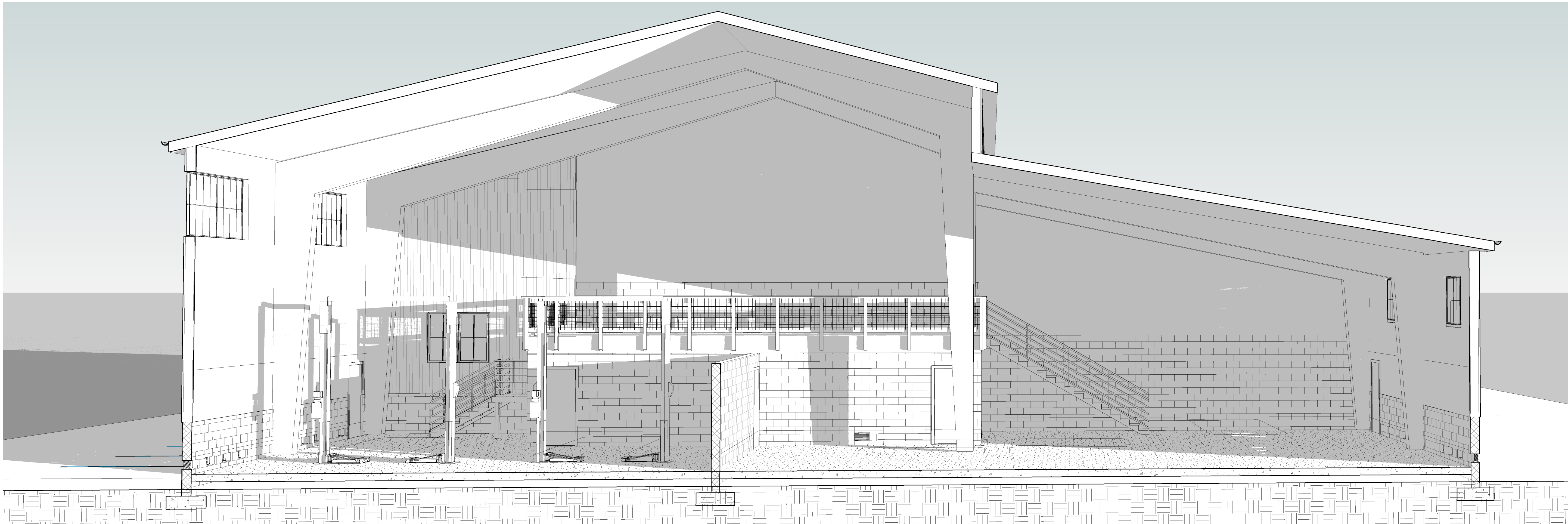
2 LONG VIEW SECT FROM NORTH
