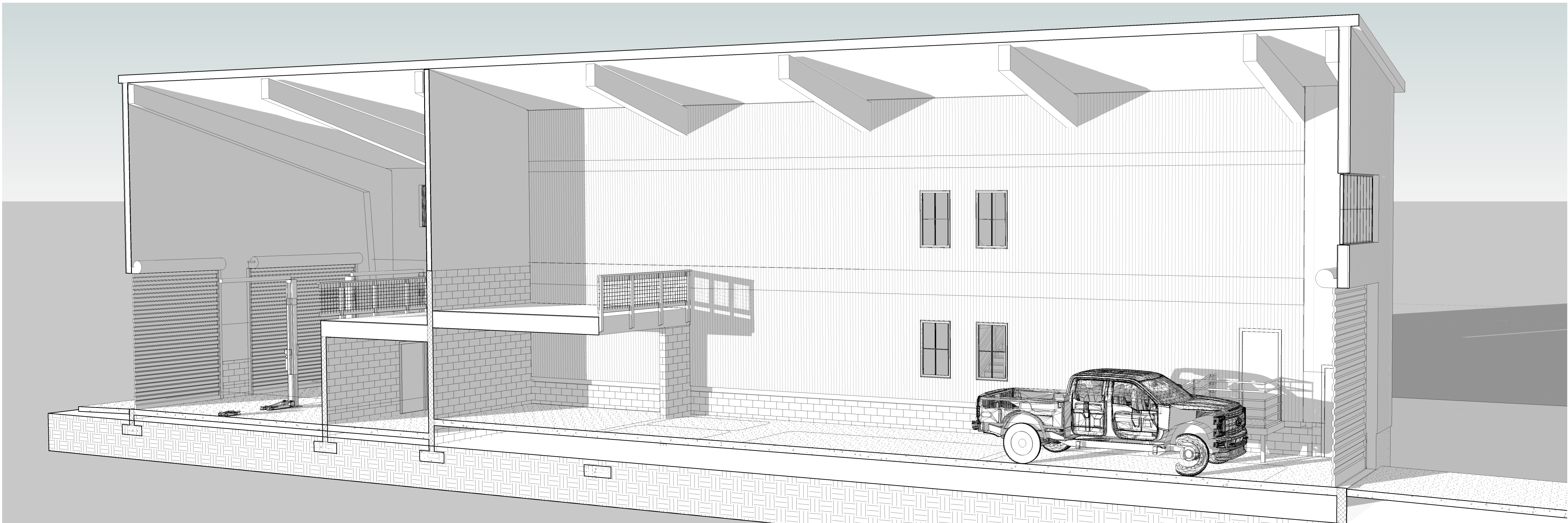
2 TRAN VIEW SECT FROM WEST 02
